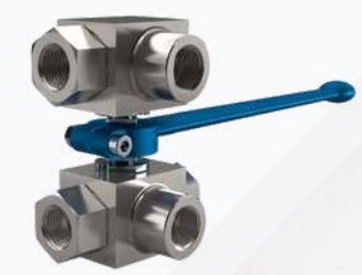
3 Way Ball Valve
